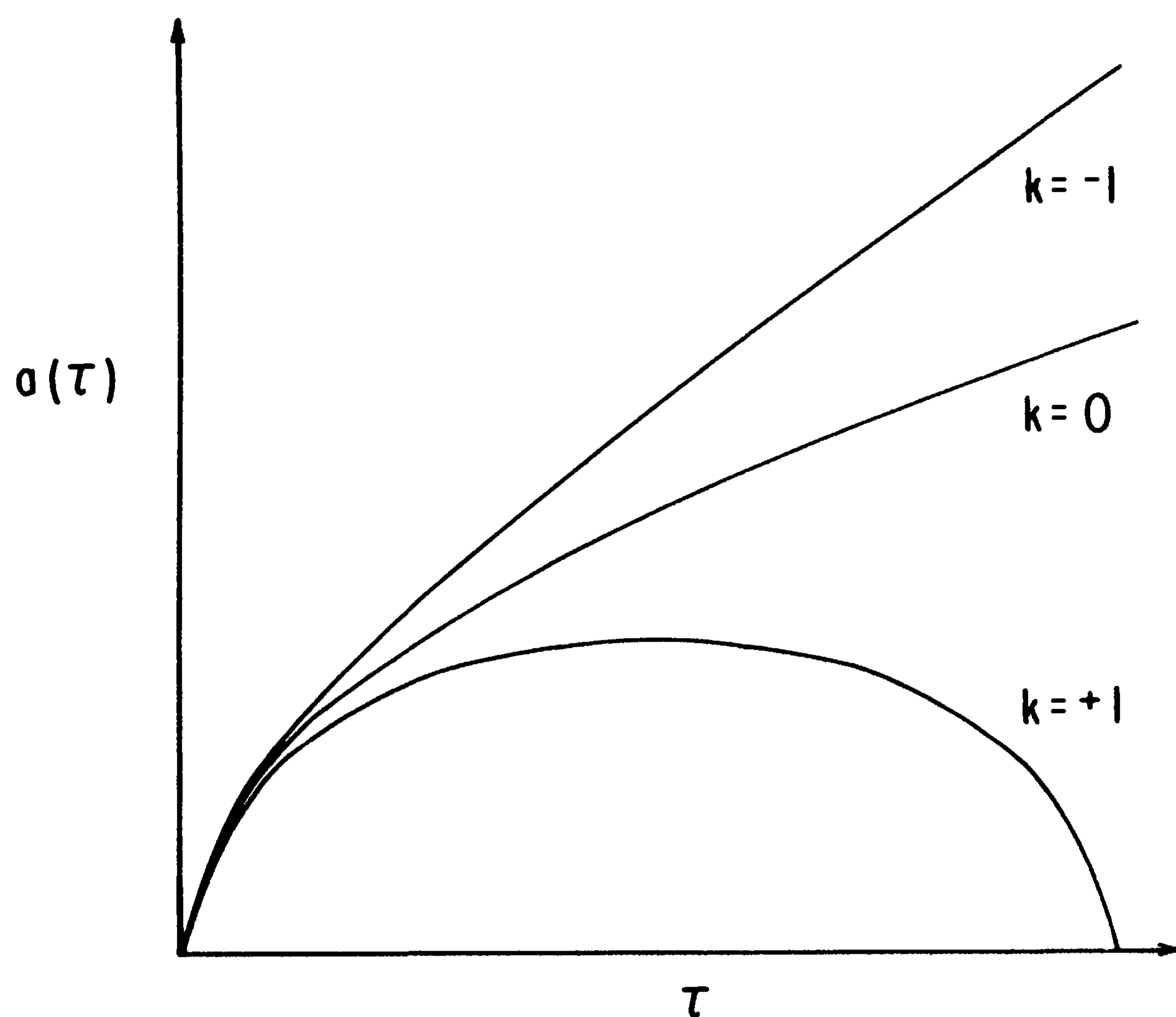
Fig. 5.3. The dynamics of dust-filled Robertson-Walker universes.
