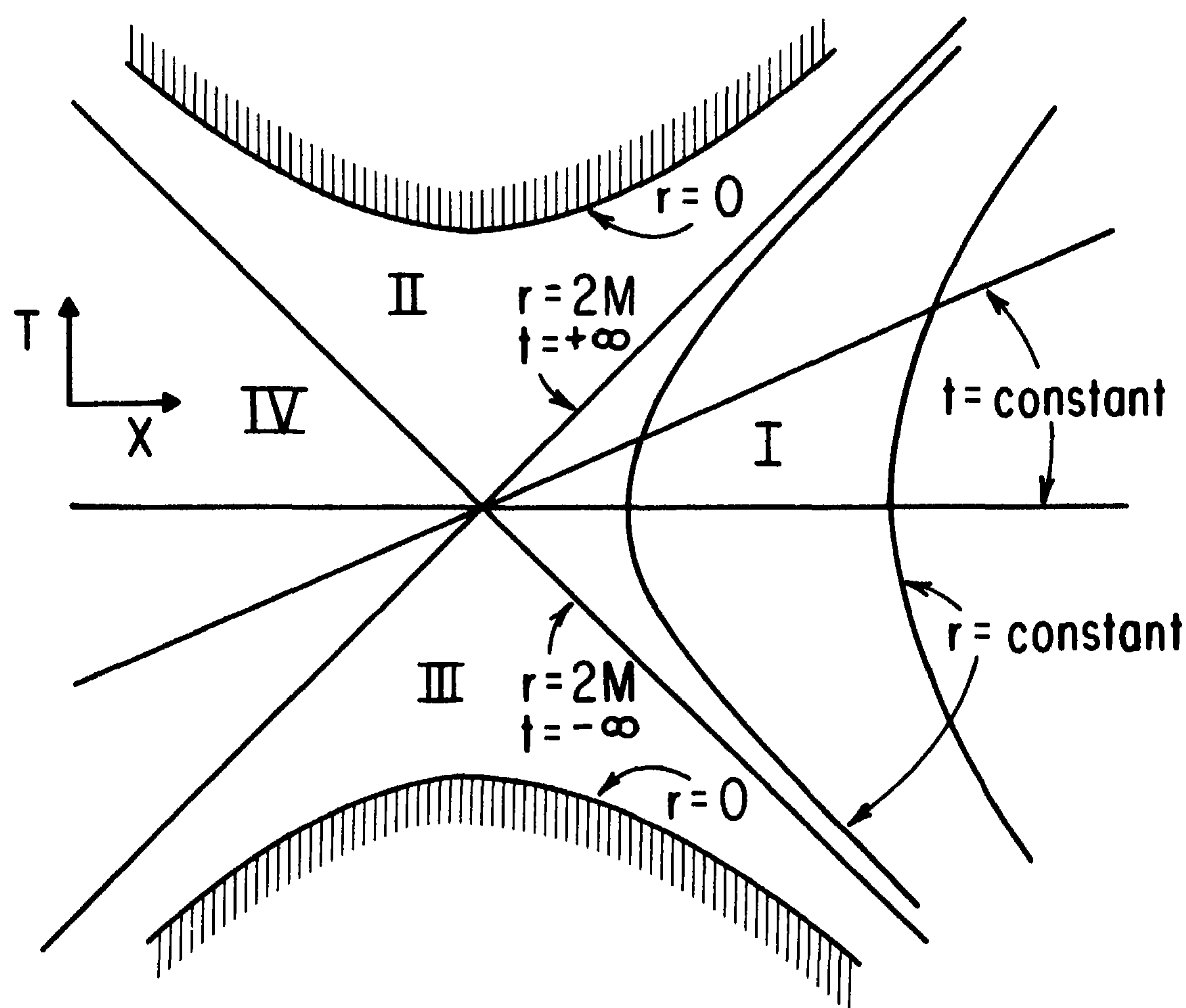
Fig. 6.9. The Kruskal extension of Schwarzschild spacetime.
