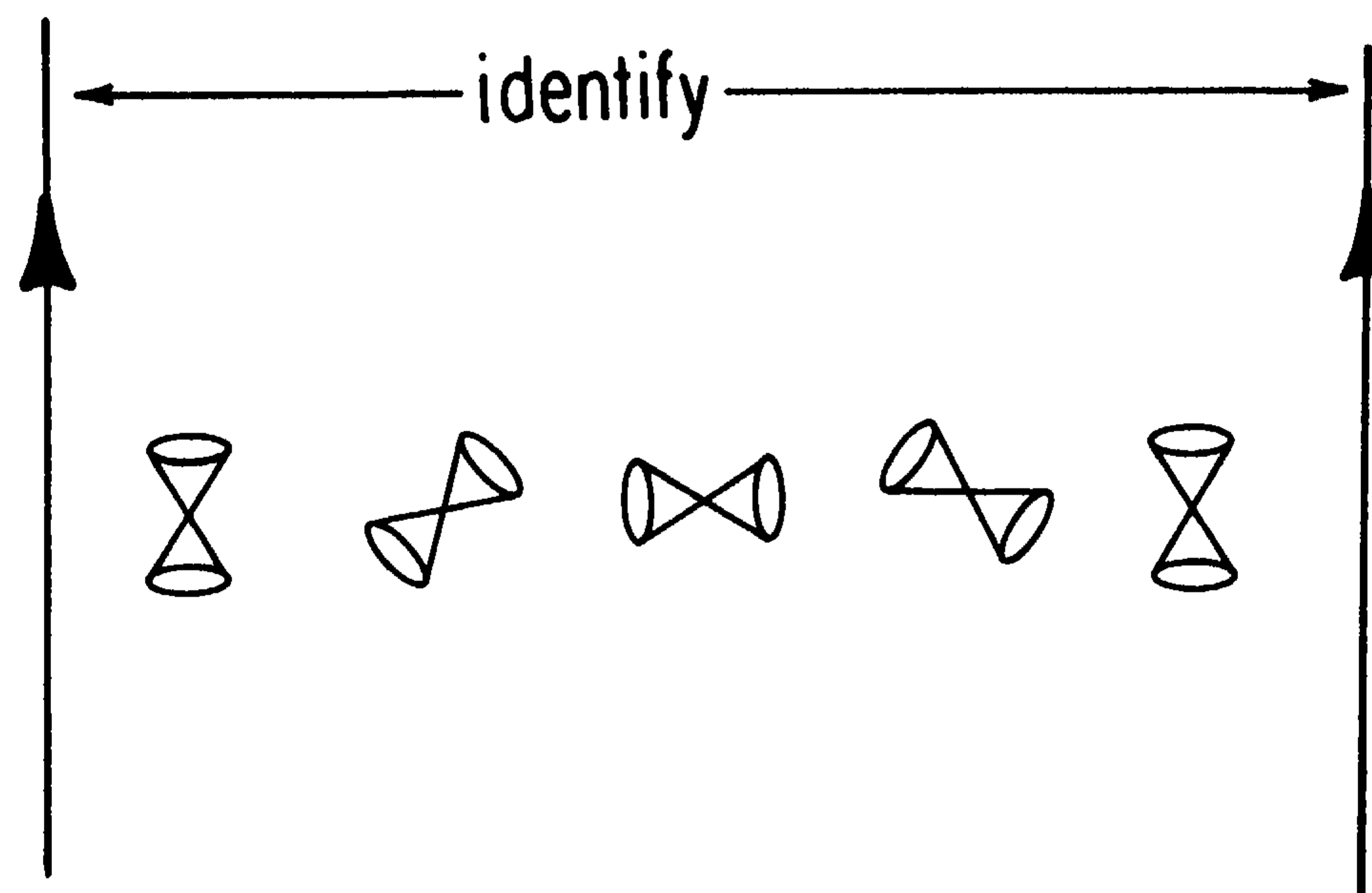
Fig. 8.1. A non-time-orientable spacetime.
