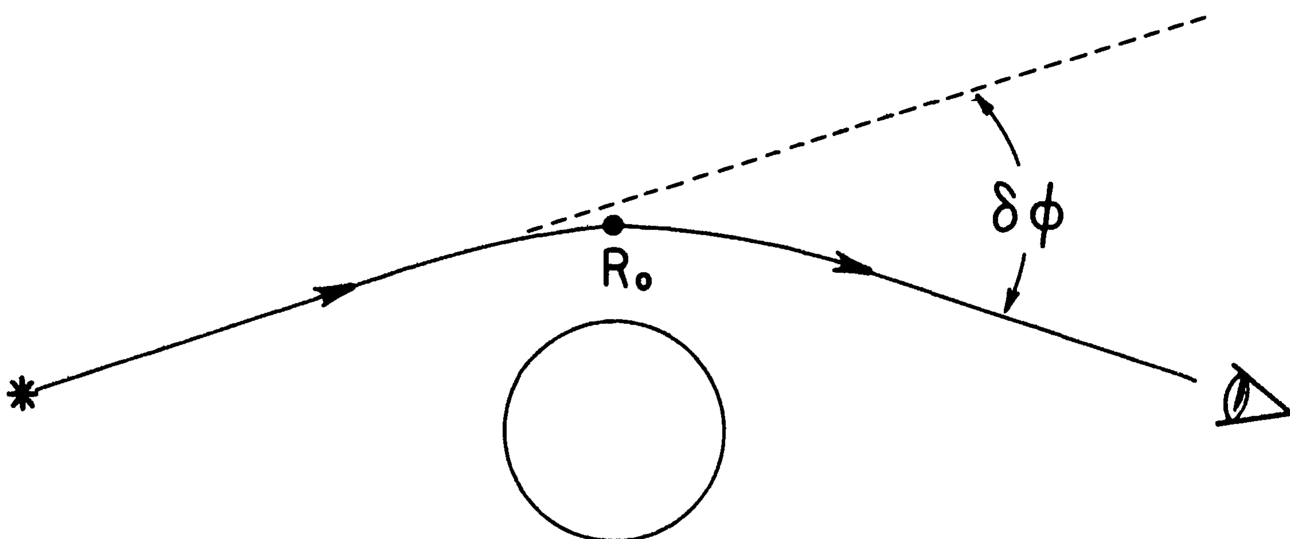
Fig. 6.6. Diagram illustrating the “bending of light” effect.
