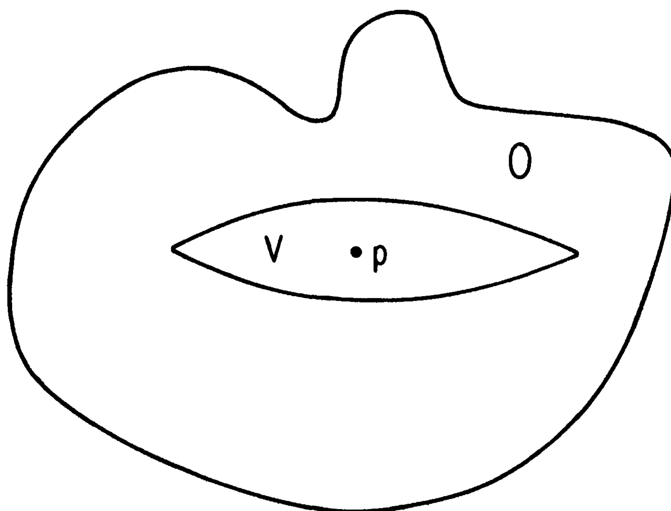
Fig. 8.9. The neighborhood, V , of p used in the proof of the corollary to theorem 8.2.2.
