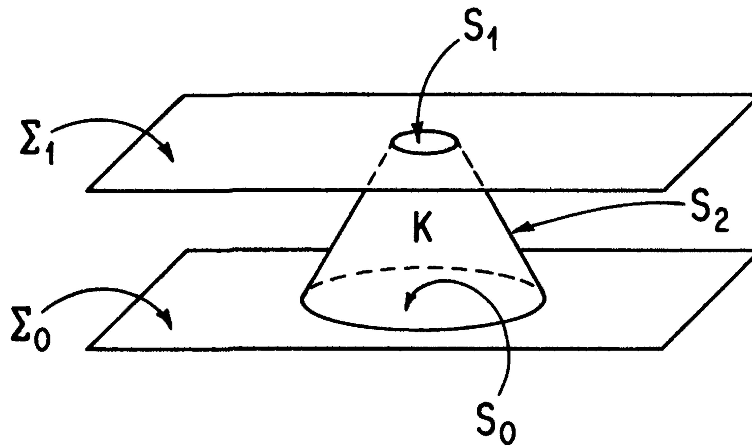
Fig. 10.1. A spacetime diagram showing the region K over which eq. (10.1.9) is integrated to obtain equation (10.1.10).
