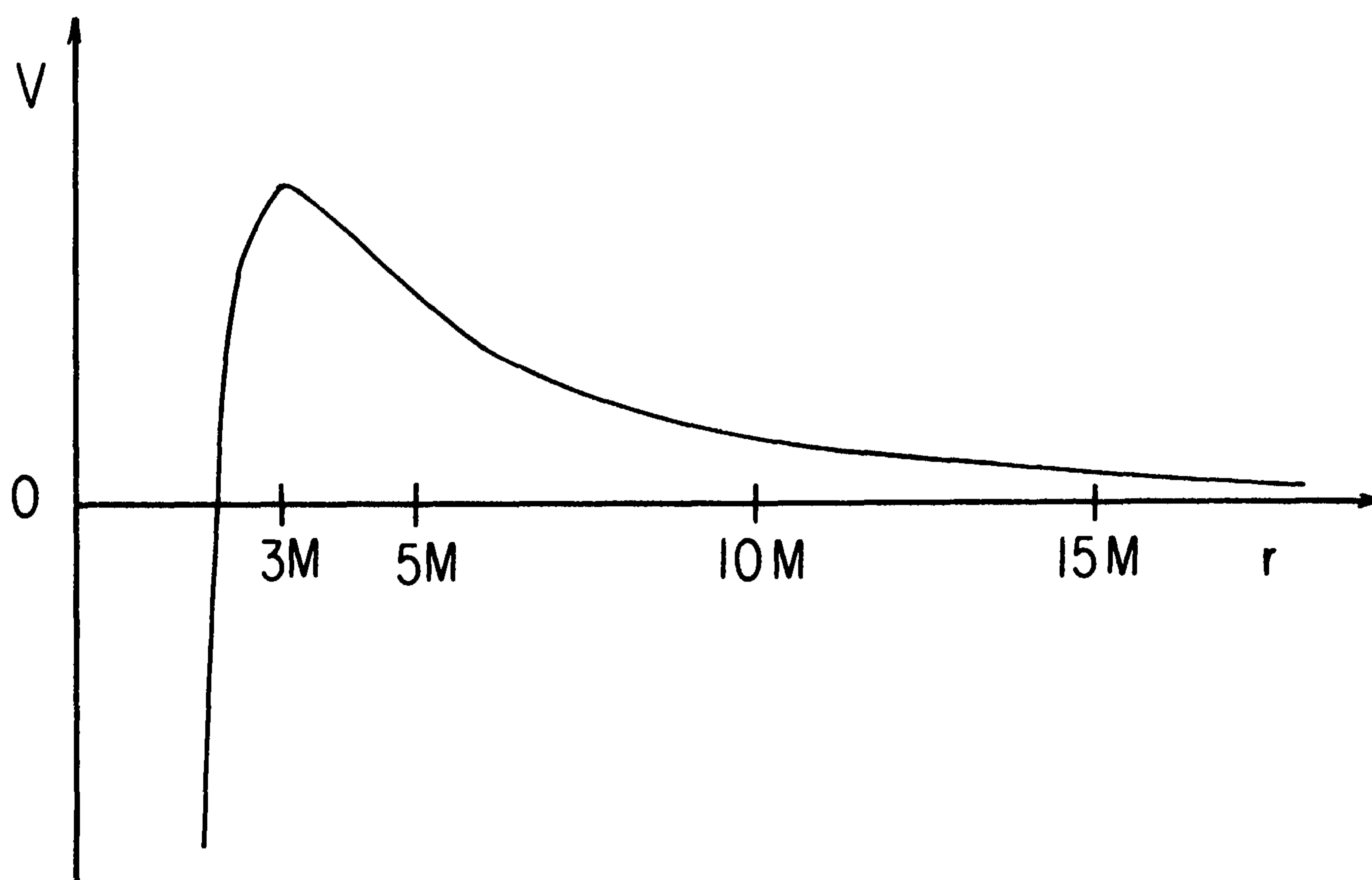
Fig. 6.5. The effective potential, V , for null geodesics.
