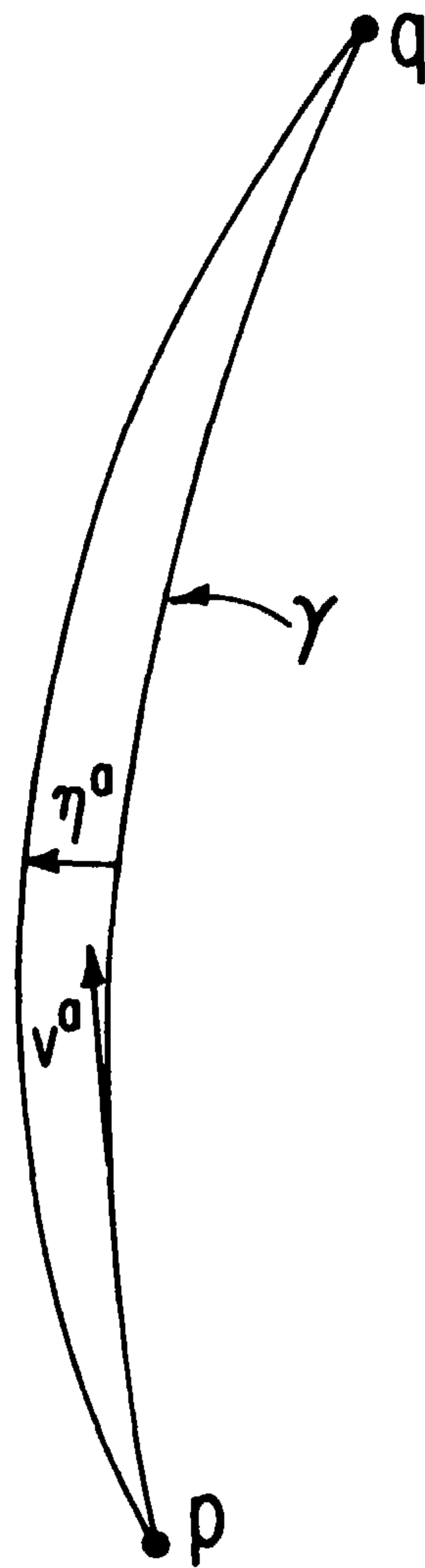
Fig. 9.2. A spacetime diagram illustrating the notion of conjugate points along the geodesic \gamma .
