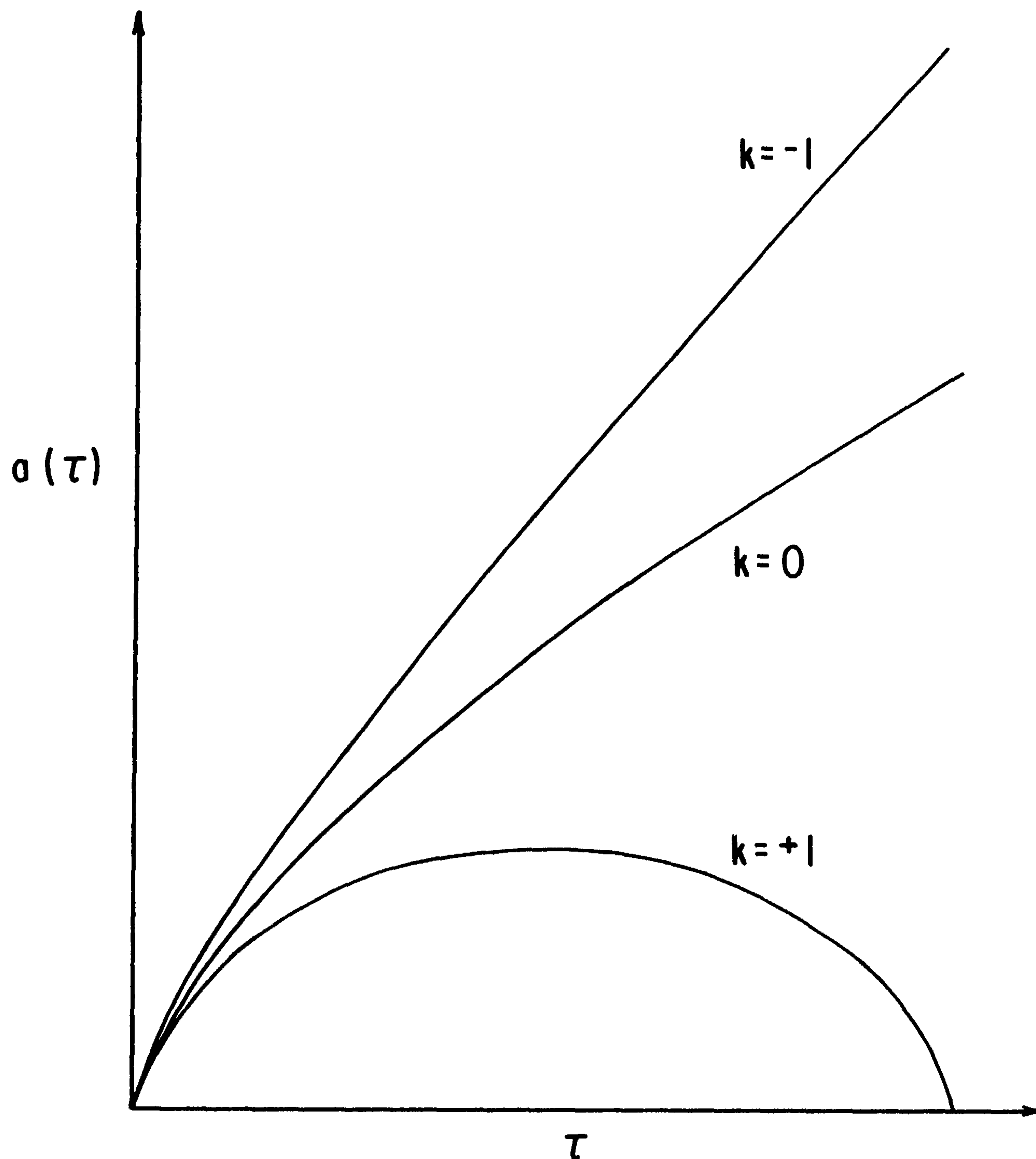
Fig. 5.4. The dynamics of radiation-filled Robertson-Walker universes.
