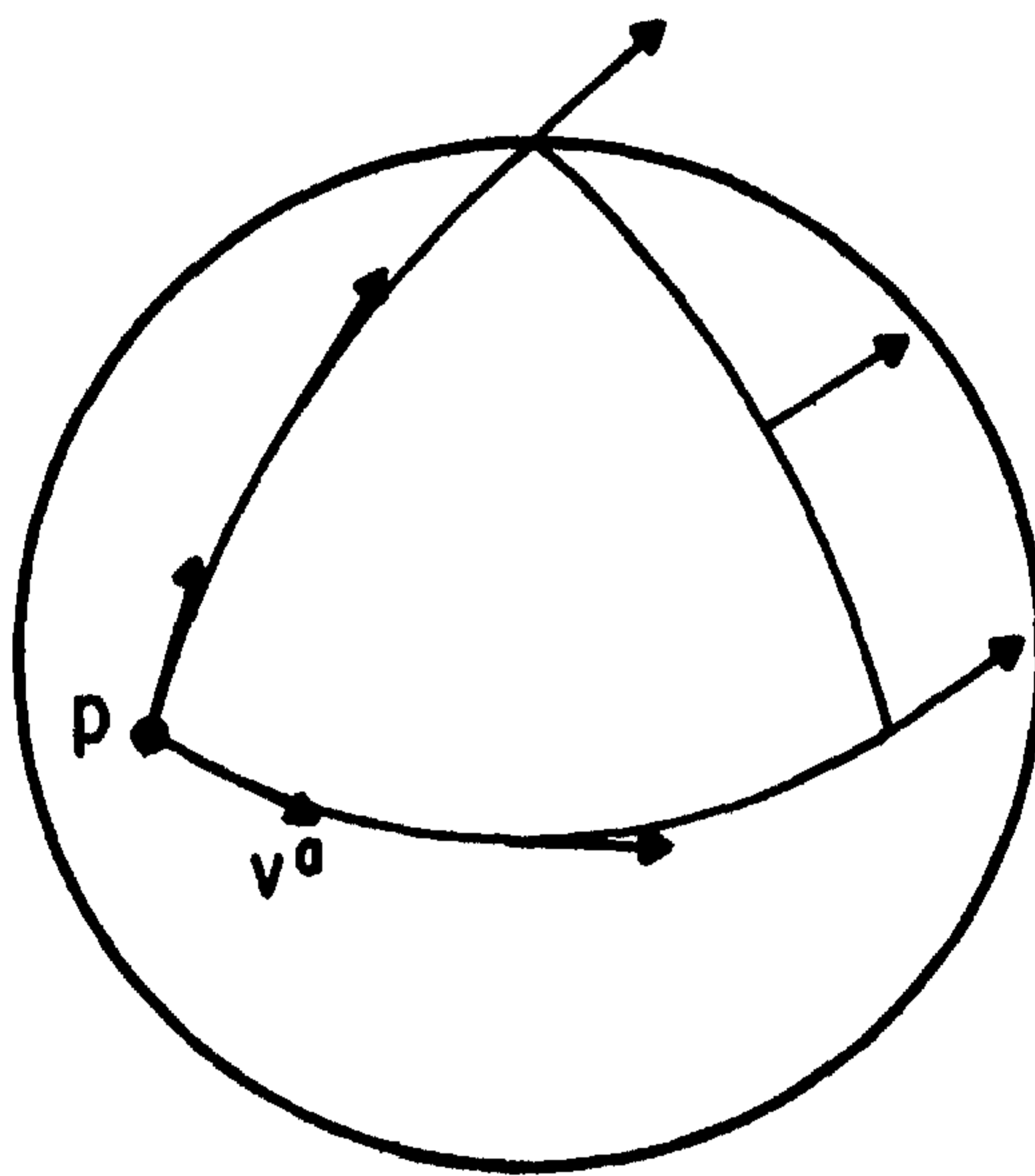
Fig. 3.2. The parallel transport of a vector, v^a , around a closed curve on the sphere. In the case shown here of a closed curve composed of three mutually orthogonal segments of great circles, the vector v^a comes back rotated by 90^\circ .
