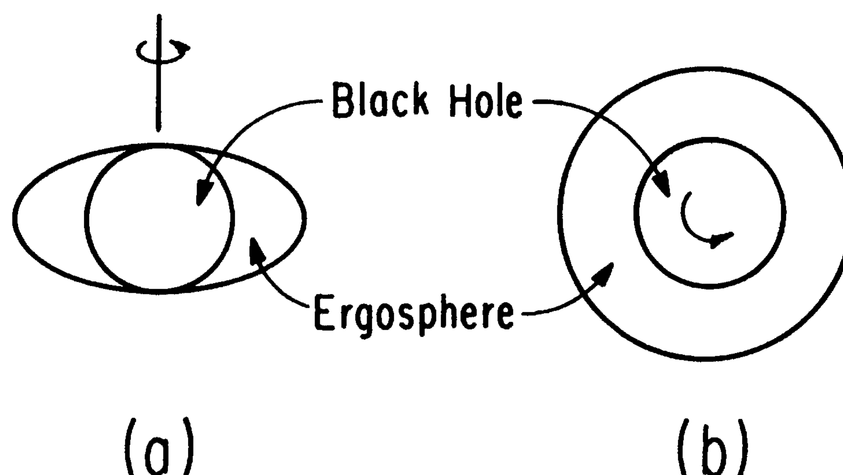
Fig. 12.6. A sketch showing (a) a “side view” and (b) a “top view” of the ergosphere of a Kerr black hole.
